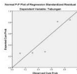
Gambar Normal P-P Plot
